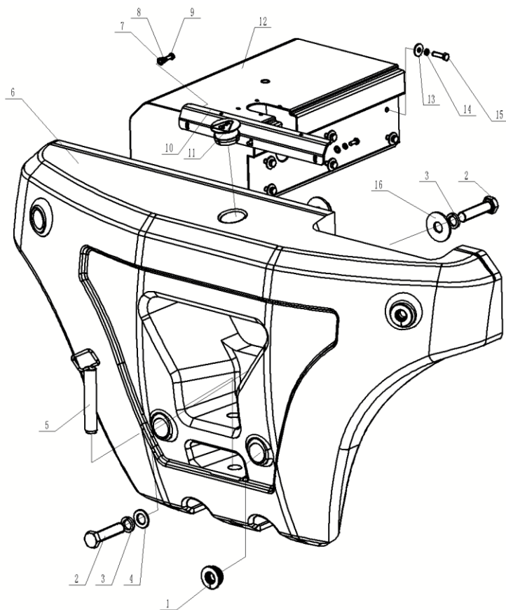
MTF25/30
